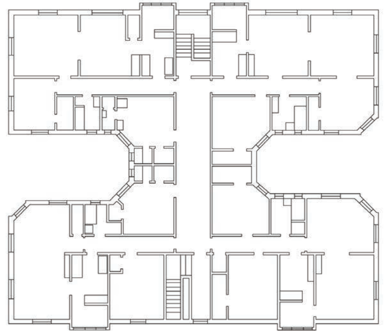
THRID FLOOR
